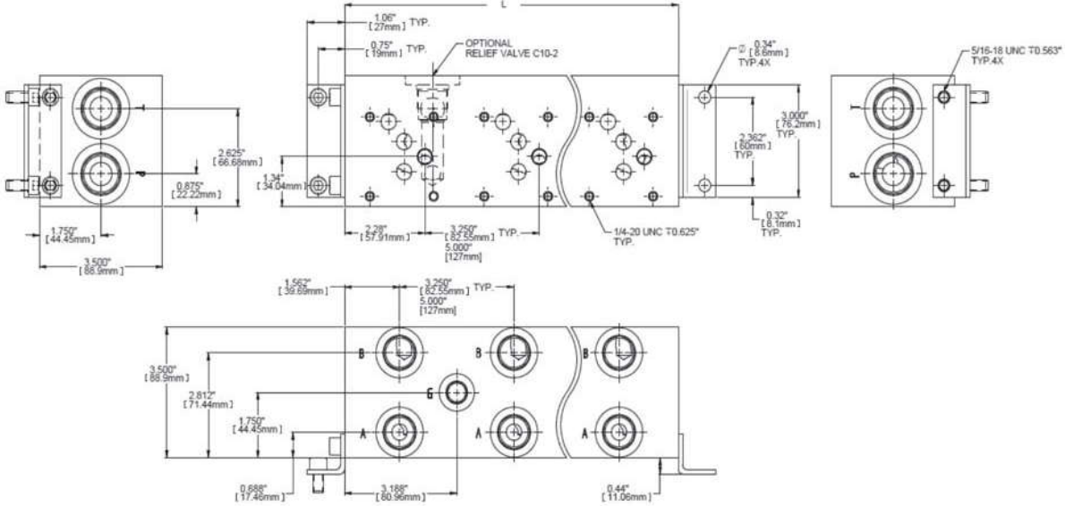
SERIES CIRCUIT WITH OPTIONAL RELIEF VALVE SHOWN
