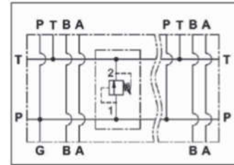
PARALLEL CIRCUIT WITH OPTIONAL RELIEF VALVE SHOWN
